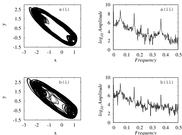
FIG. 10. Projection of the numerically simulated attractors of Eqs. (2) in the (x,y) plane for fixed E_1=0.34 and various values of a indicating the transition from quasiperiodic attractor to SNA through fractalization route: (a) period-3 torus (3T) for a=0.954\ 406 and (b) SNA at a=0.954\ 351 : (i) phase trajectory in the (x-y) plane; (ii) power spectrum.
