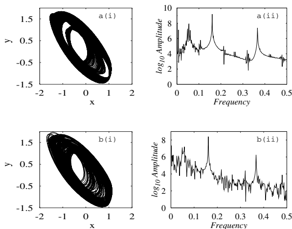
FIG. 16. Projection of the numerically simulated attractors of Eqs. (2) for fixed E_1=0.635 and two different values of a indicating the transition from quasiperiodic attractor to SNA through type-I intermittent route: (a) period-3 torus (3T) for a=0.951912 and (b) SNA at a=0.951889 ; (i) phase trajectory in the (x-y) plane; (ii) power spectrum.
