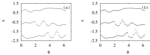
FIG. 9. Projection of the numerically simulated attractors of Eqs. (2) in the (\phi-x) plane for fixed E_1=0.34 and various values of a indicating the transition from quasiperiodic attractor to SNA through fractalization route. (a) period-3 torus (3T) for a=0.954\ 406 and (b) SNA at a=0.954\ 351 .
