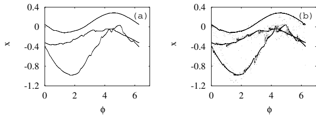
FIG. 15. Projection of the simulated attractors of Eqs. (2) in the (\phi-x) plane for fixed E_1=0.635 and various value of a : indicating the transition from quasiperiodic attractor to SNA through type-I intermittent route. (a) torus (3T) for a=0.951912 and (b) SNA at a=0.951889 .
