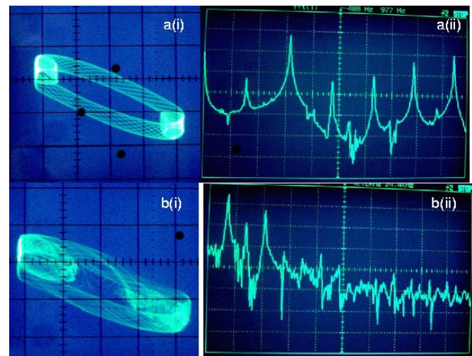
FIG. 12. (Color online) Attractors obtained experimentally from the circuit given in Fig. 1 corresponding to Figs. 10. (a) period-3 torus (3T) for R=2102\ \Omega and (b) SNA at R=2101\ \Omega for fixed value of E_{f1}=0.17\ V : (i) phase trajectory ( v-i_L ); (ii) power spectrum.
