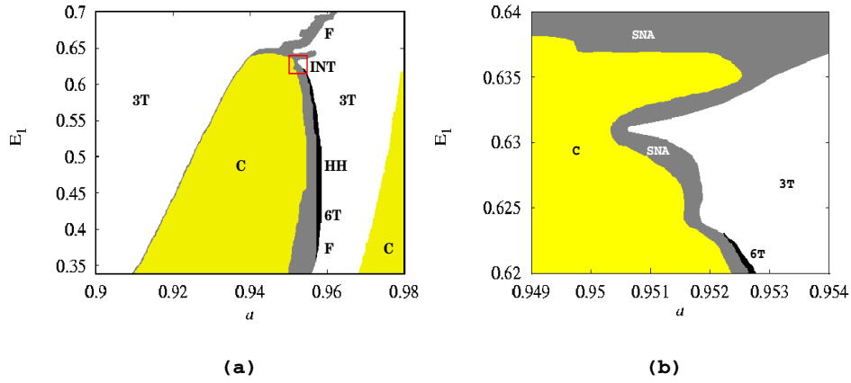
FIG. 2. (Color online) (a) Phase diagram in the (a-E_1) plane for the circuit given in Fig. 1, represented by Eq. (2) and obtained from numerical data. 3T and 6T correspond to torus of period-3 and period-6 attractors, respectively. F, HH, and INT denote the formation of SNAs through gradual fractalization, Heagy-Hammel, and intermittency routes, respectively. C corresponds to chaotic attractor. (b) An enlarged version of the intermittent region is indicated in (a).
