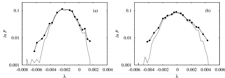
FIG. 14. Distribution of finite-time Lyapunov exponents on SNAs created through gradual fractalization: (a) quasiperiodic attractor, (b) strange nonchaotic attractor. Finite-time Lyapunov exponents calculated from numerical data are indicated by dashed lines, and from experimental data are denoted by solid lines.
