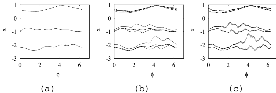
FIG. 3. Projection of the numerically simulated attractors of Eqs. (2) in the (\phi-x) plane for fixed E_1=0.44 and various values of a indicating the transition from quasiperiodic attractor to SNA through the Heagy-Hammel mechanism: (a) period-3 torus (3T) for a=0.956\ 32, (b) period-6 torus (6T) for a=0.955\ 93, and (c) SNA at a=0.955\ 92.
