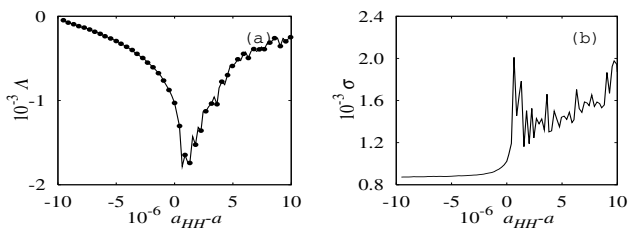
FIG. 5. Transition from three doubled torus to SNA through Heagy-Hammel route in region HH obtained from numerical data: (a) the behavior of the maximal Lyapunov exponent ( \Lambda ) and (b) the variance ( \sigma ) for E_1=0.44 .
