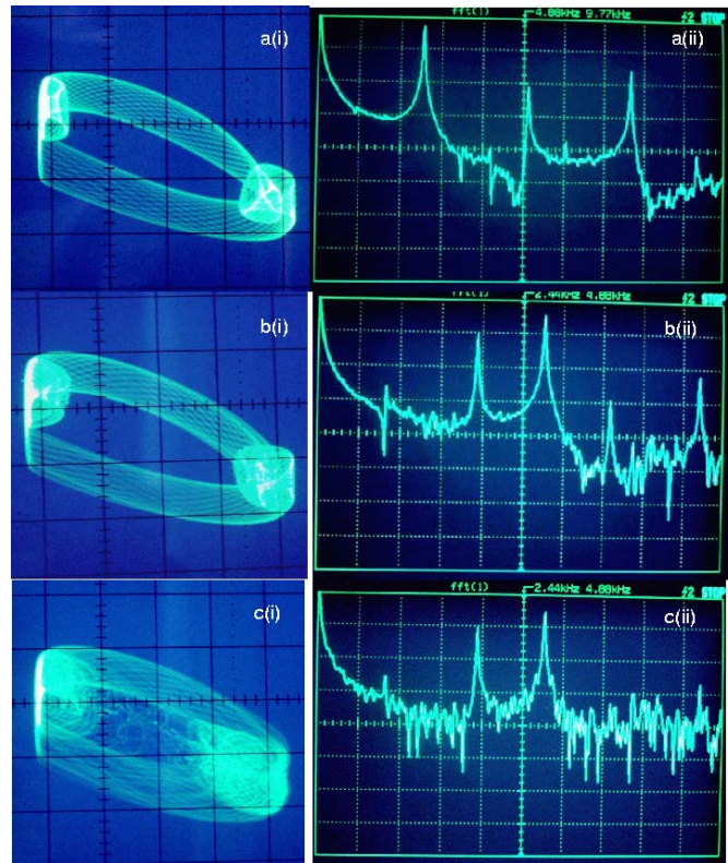
FIG. 6. (Color online) Attractors obtained experimentally from the circuit given in Fig. 1 corresponding to Figs. 4. (a) period-3 torus (3T) for R=2109 \Omega , (b) period-6 torus (6T) for R=2106 \Omega , and (c) SNA at R=2104 \Omega for fixed value of E_{f1}=0.22 V: (i) phase trajectory in the (v-i_L) space; (ii) power spectrum.
