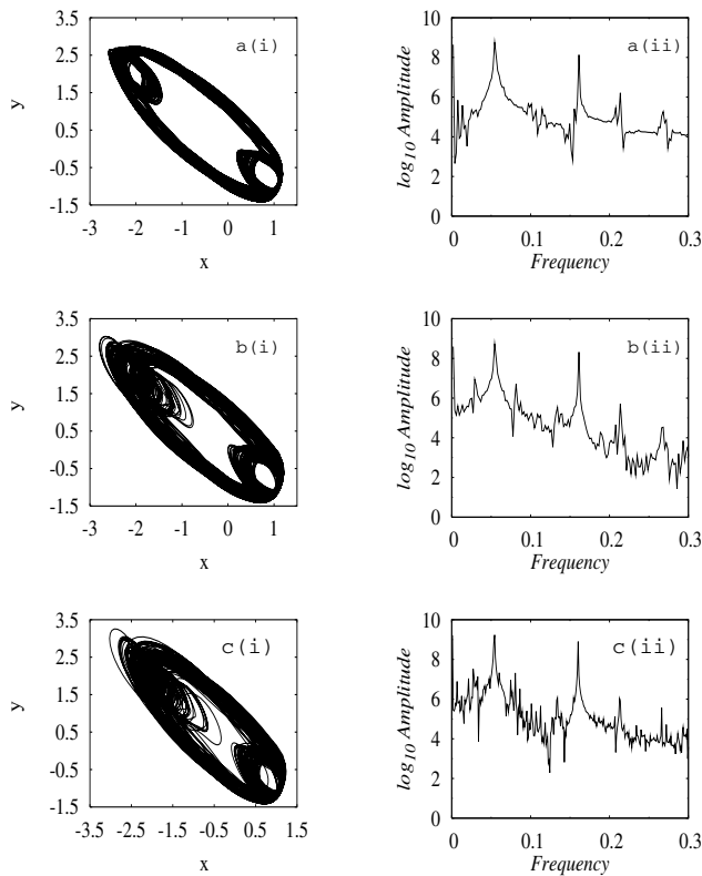
FIG. 4. Projection of the numerically simulated attractors of Eqs. (2) in the (x, y) plane for fixed E_1=0.44 and various values of a indicating the transition from a quasiperiodic attractor to an SNA through the Heagy-Hammel route: (a) period-3 torus (3T) for a=0.95632 , (b) period-6 torus (6T) for a=0.95593 , and (c) SNA at a=0.95592 : (i) phase trajectory in the (x-y) space; (ii) power spectrum.
