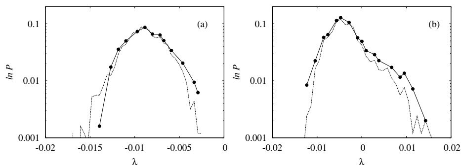
FIG. 21. Distribution of finite-time Lyapunov exponents on SNAs created through type-I intermittency. (a) quasiperiodic attractor, (b) strange nonchaotic attractor. Finite-time Lyapunov exponents calculated from numerical data are indicated by dashed lines, and from experimental data are denoted by solid lines.
