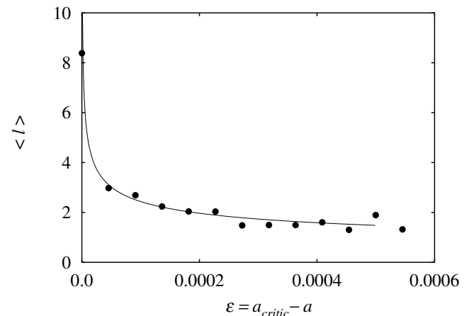
FIG. 18. Average laminar length ( \langle l \rangle ) vs (a_{critic}-a) at a_{critic}=0.951876 obtained from numerical data.
