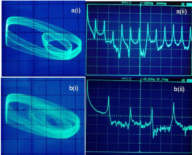
FIG. 19. (Color online) Attractors obtained experimentally from the circuit given in Fig. 1 corresponding to Figs. 16. (a) period-3 torus (3T) for R=2099 \Omega and (b) SNA at R=2097 \Omega for fixed value of E_{f1}=0.318 \text{ V} : (i) phase trajectory ( v-i_L ); (ii) power spectrum.
